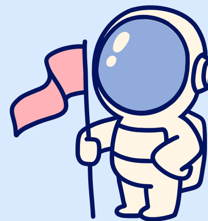
Astronauta
